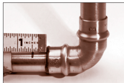
FIGURE 88: Ensuring proper insertion depth
