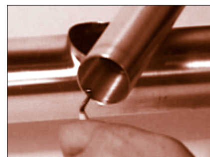
FIGURE 99: Reaming the branch tube end
