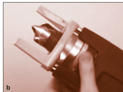
FIGURE 93 (a and b): Chucking the drill head assembly
