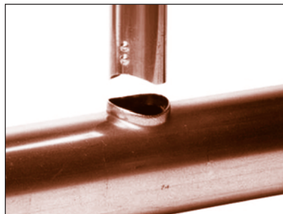
FIGURE 103: Aligning the dimples with the run of the tube
