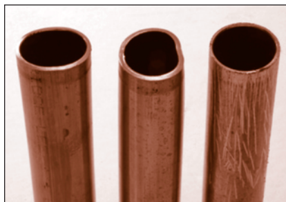
FIGURE 33: Inspect tube for imperfections
