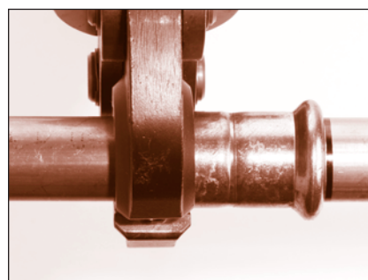
FIGURE 60: Properly positioned press tool
